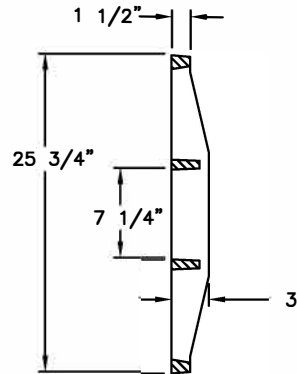
GRATE SECTION
