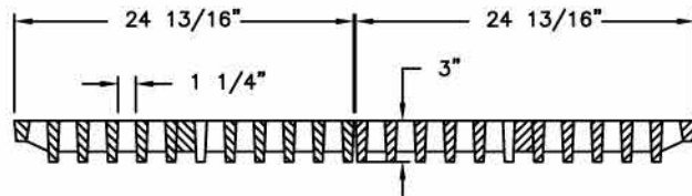
GRATE SECTION
