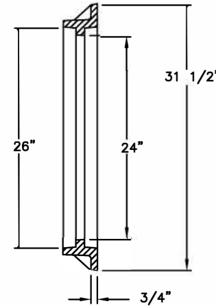
FRAME SECTION
