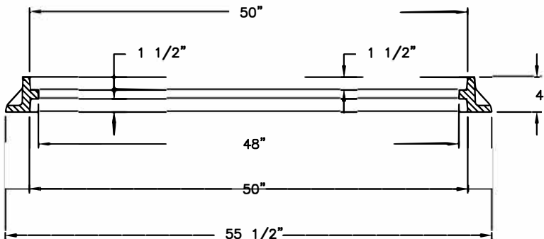
FRAME SECTION
